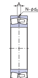
With oil holes / oil groove (W33)
