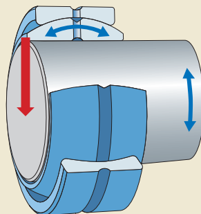
Dynamic bearing load
