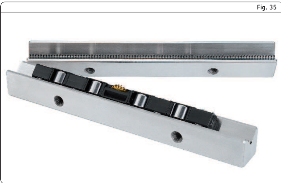
Design of an LWRE rail guide with ACSM
